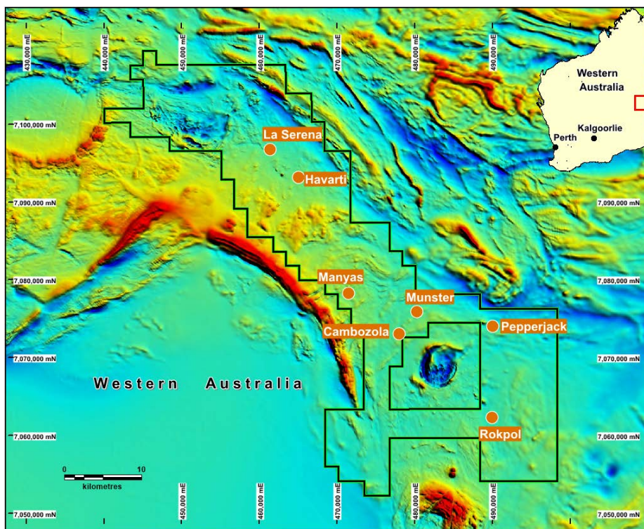
Figure 1. Aeromagnetic image of the Latitude Hill project showing the position of the Spectrem targets
